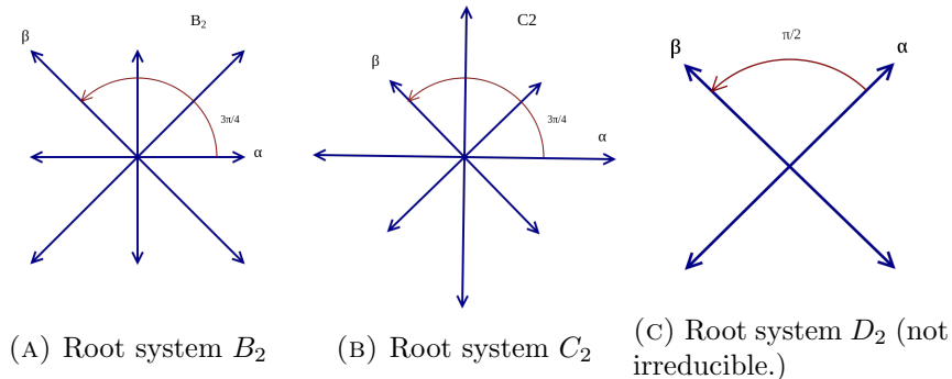
FIGURE 2. Classical irreducible root systems when n = 2 from [Wik17]
